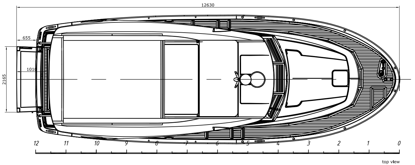
Greenline 40 - General dimensions
